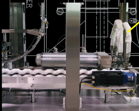
Glue Applicator
